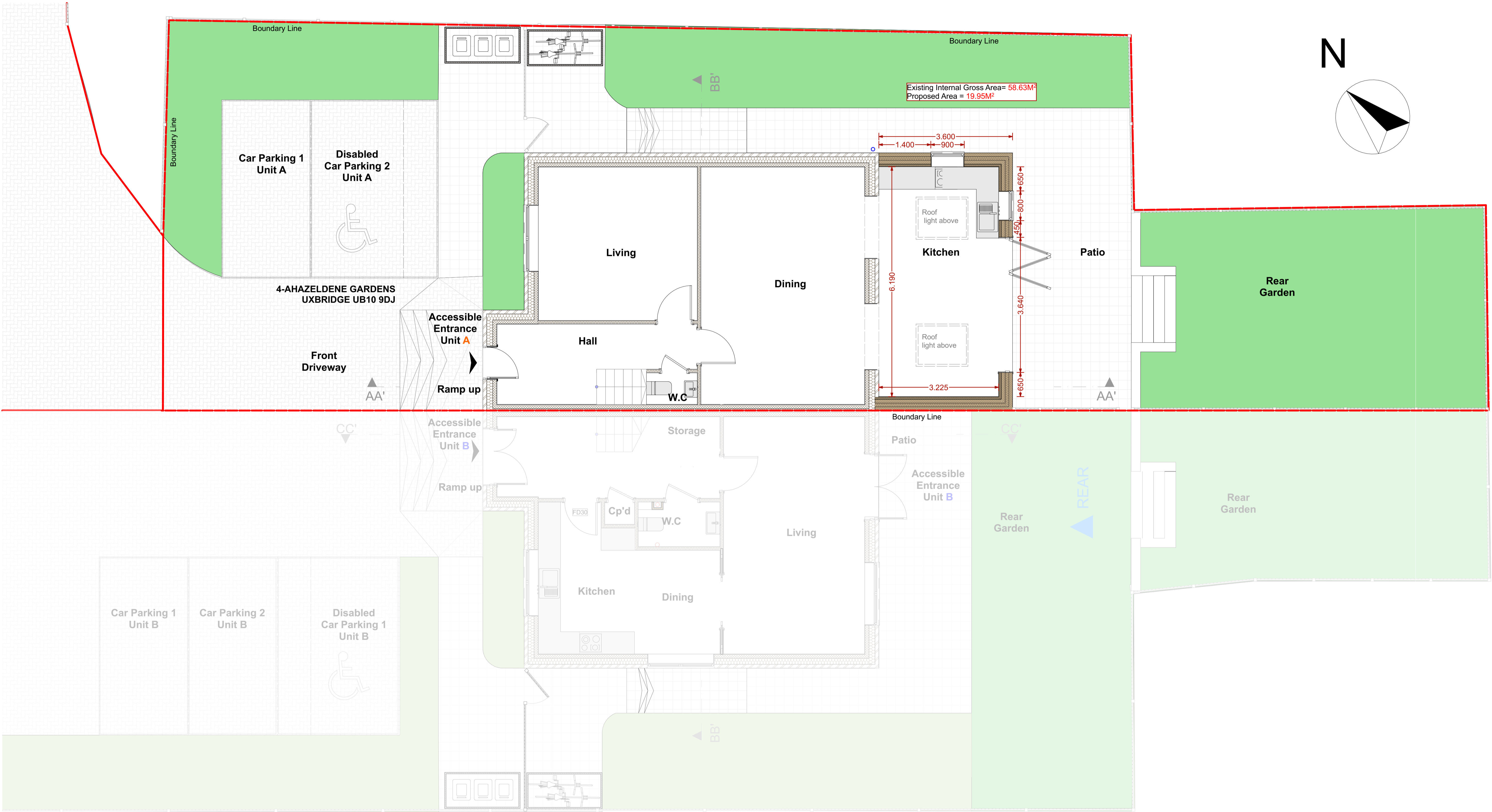
Proposed Ground Floor Plan 1:50
