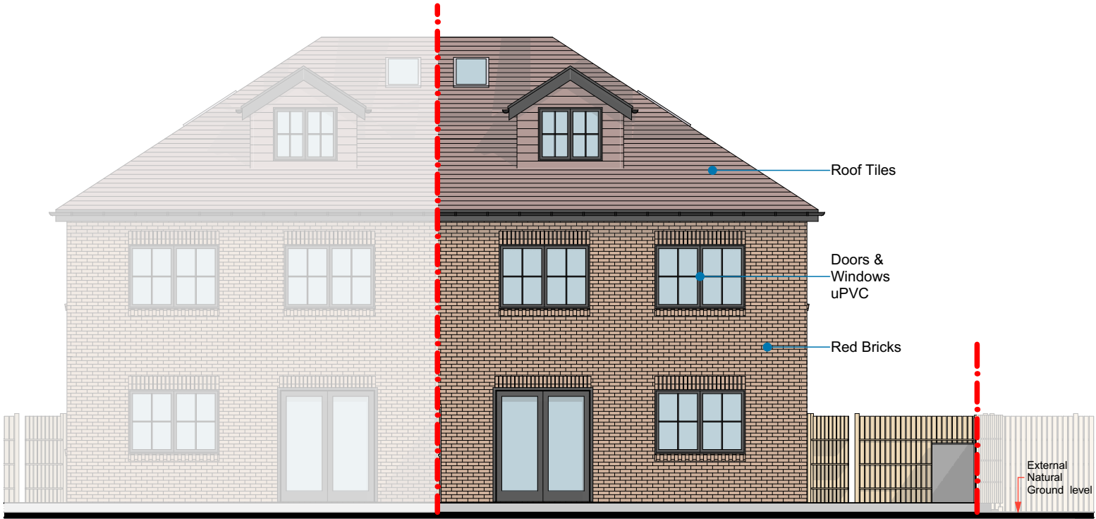
Existing Rear Elevation 1:100
