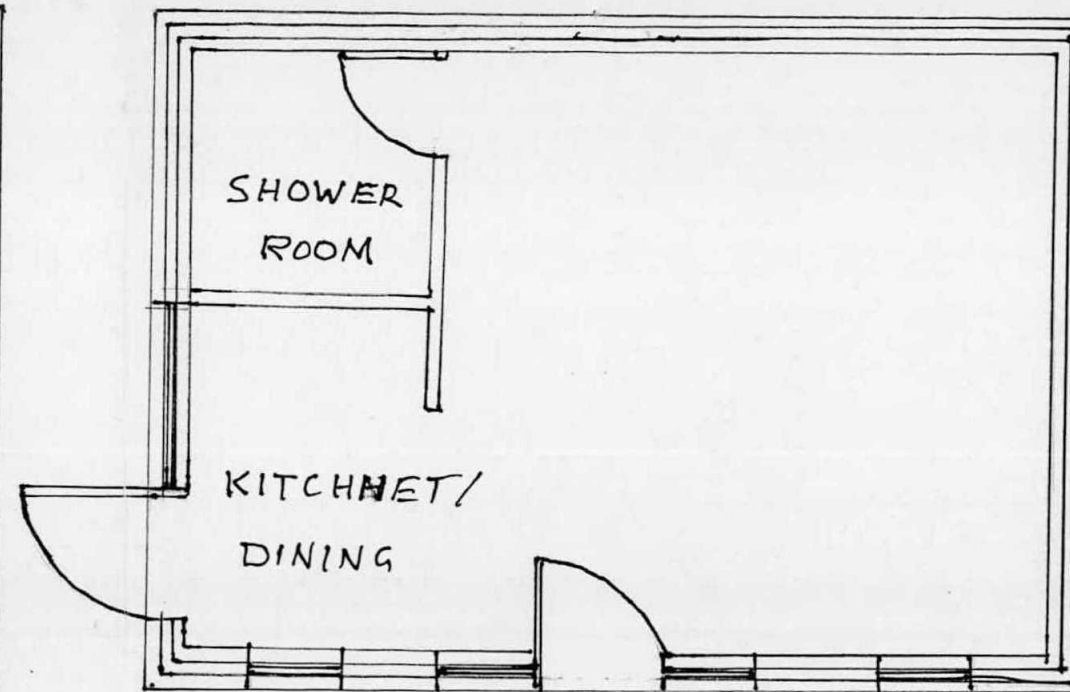
PROPOSED GRANNY ANNEXE STUDIO PLAN
