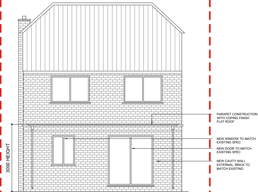
B. PROPOSED REAR ELEVATION
