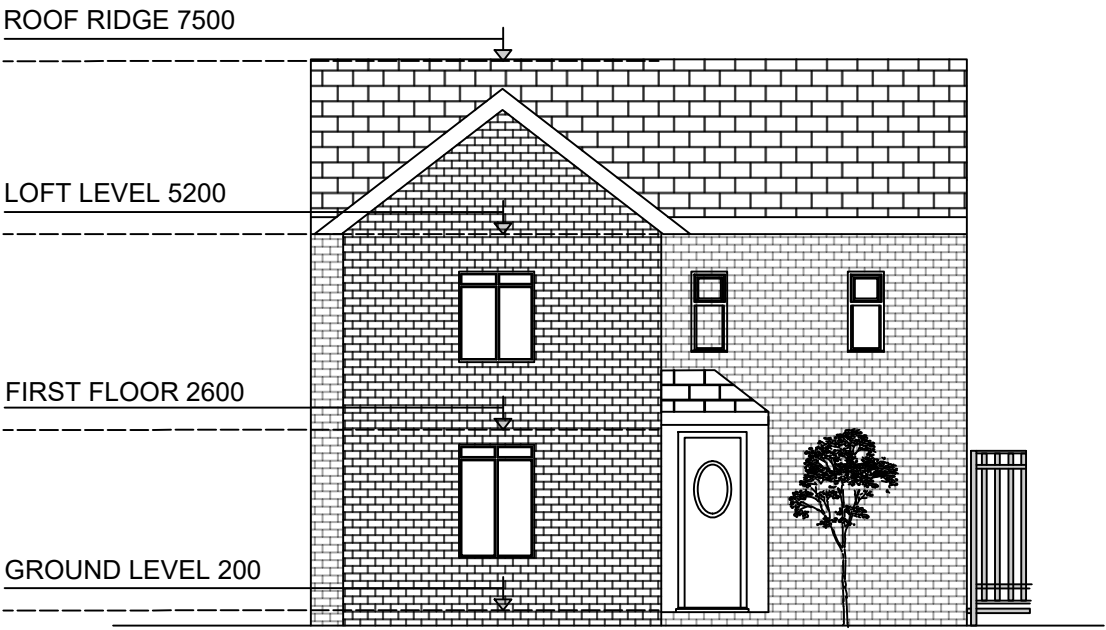
FRONT ELEVATION
