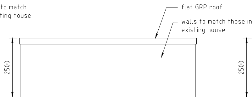
PROPOSED ELEVATION B
