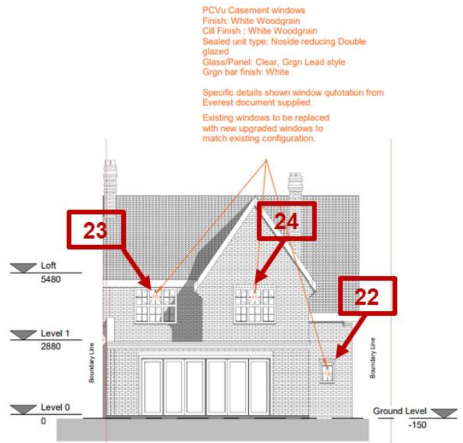
Rear elevation - Proposed 1 : 100
