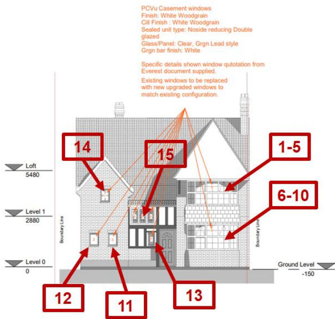
Front elevation - Proposed 1 : 100
