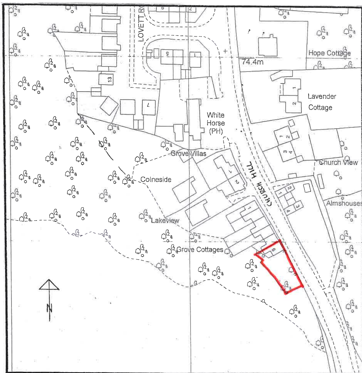
SITE LOCATION 1:1250
