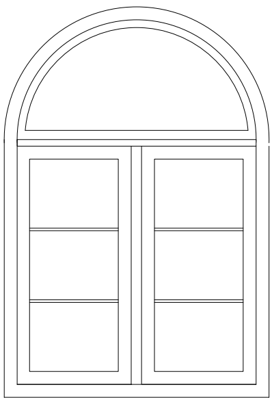
1025 x 1000 (fixed light with fanlight over)
