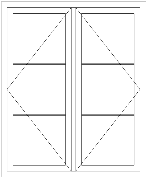
1240 x 1500 (double casement)
