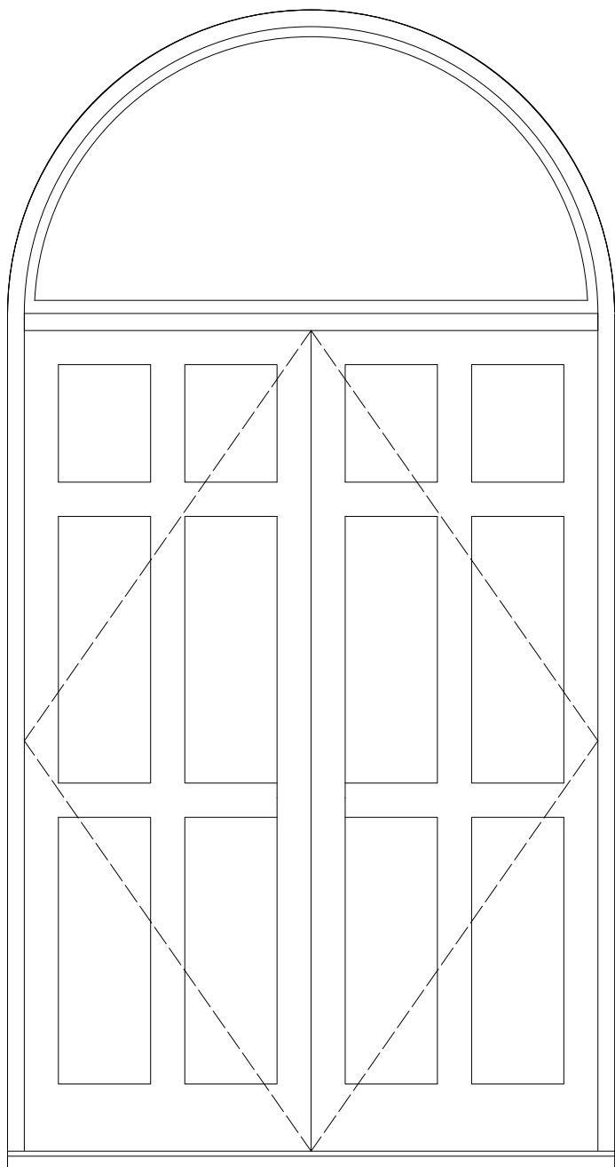
1800 x 2550 (front door with fanlight)
