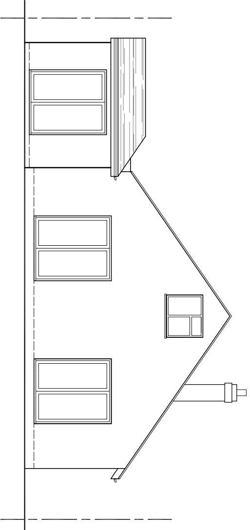
NORTH ELEVATION
