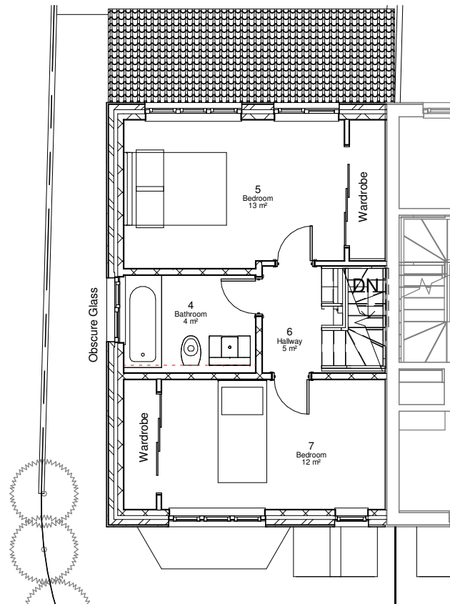
2 First Floor 1 : 100
