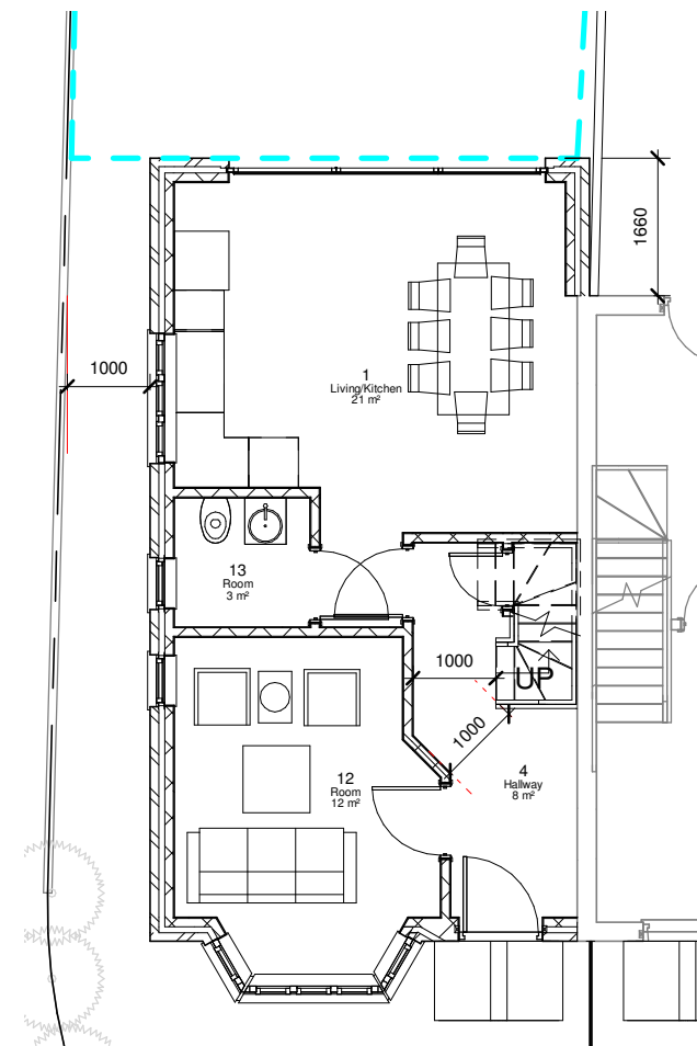
1 Ground Floor 1 : 100
