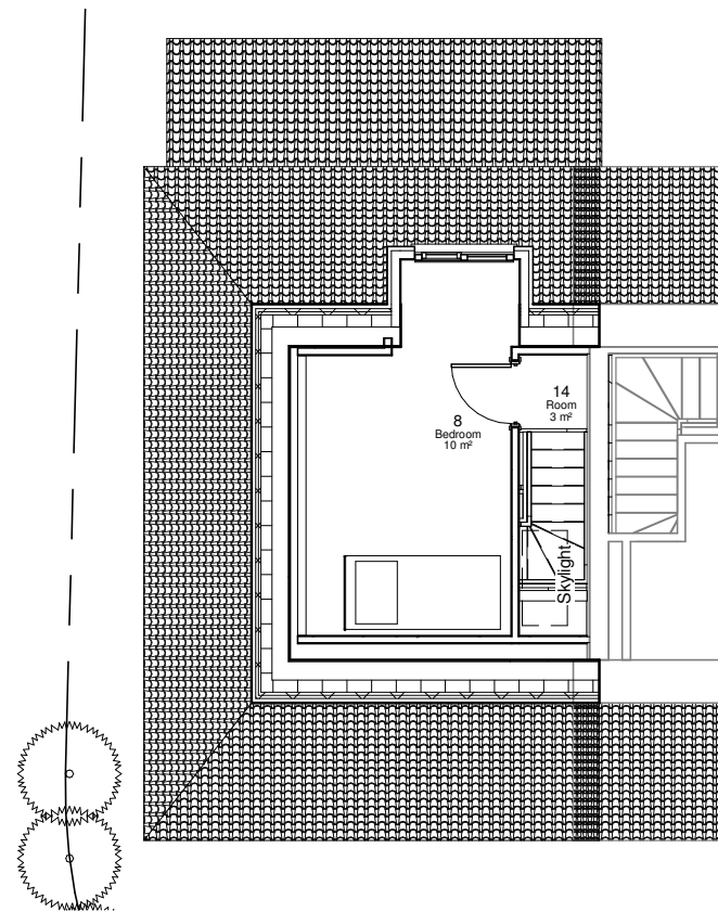
3 Second Floor 1 : 100
