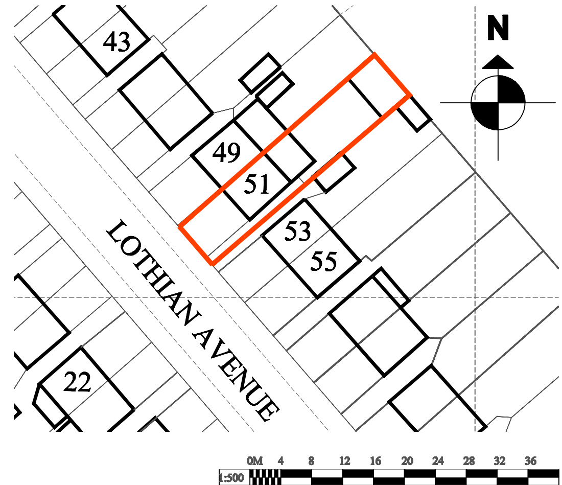
BLOCK PLAN 1:500
