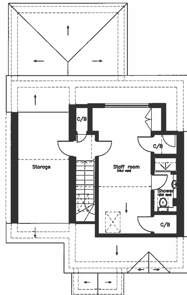
PROPOSED LOFT
