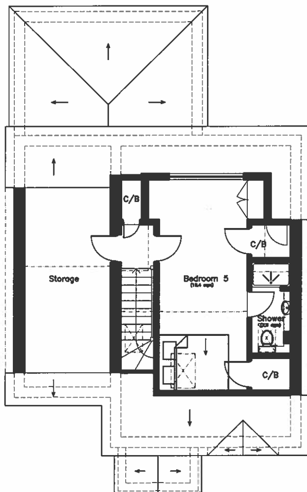
EXISTING LOFT
