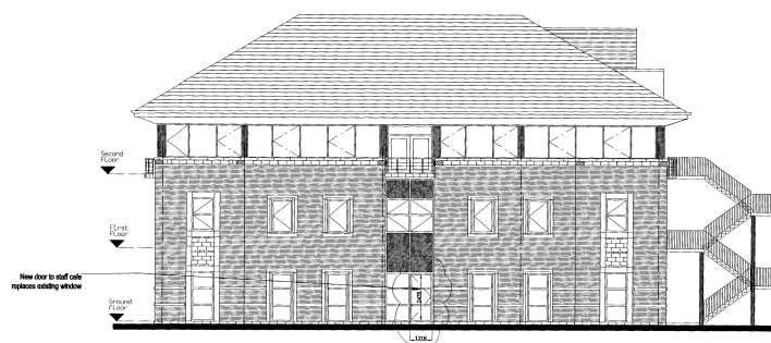
East Elevation- Door Replaces Window.
