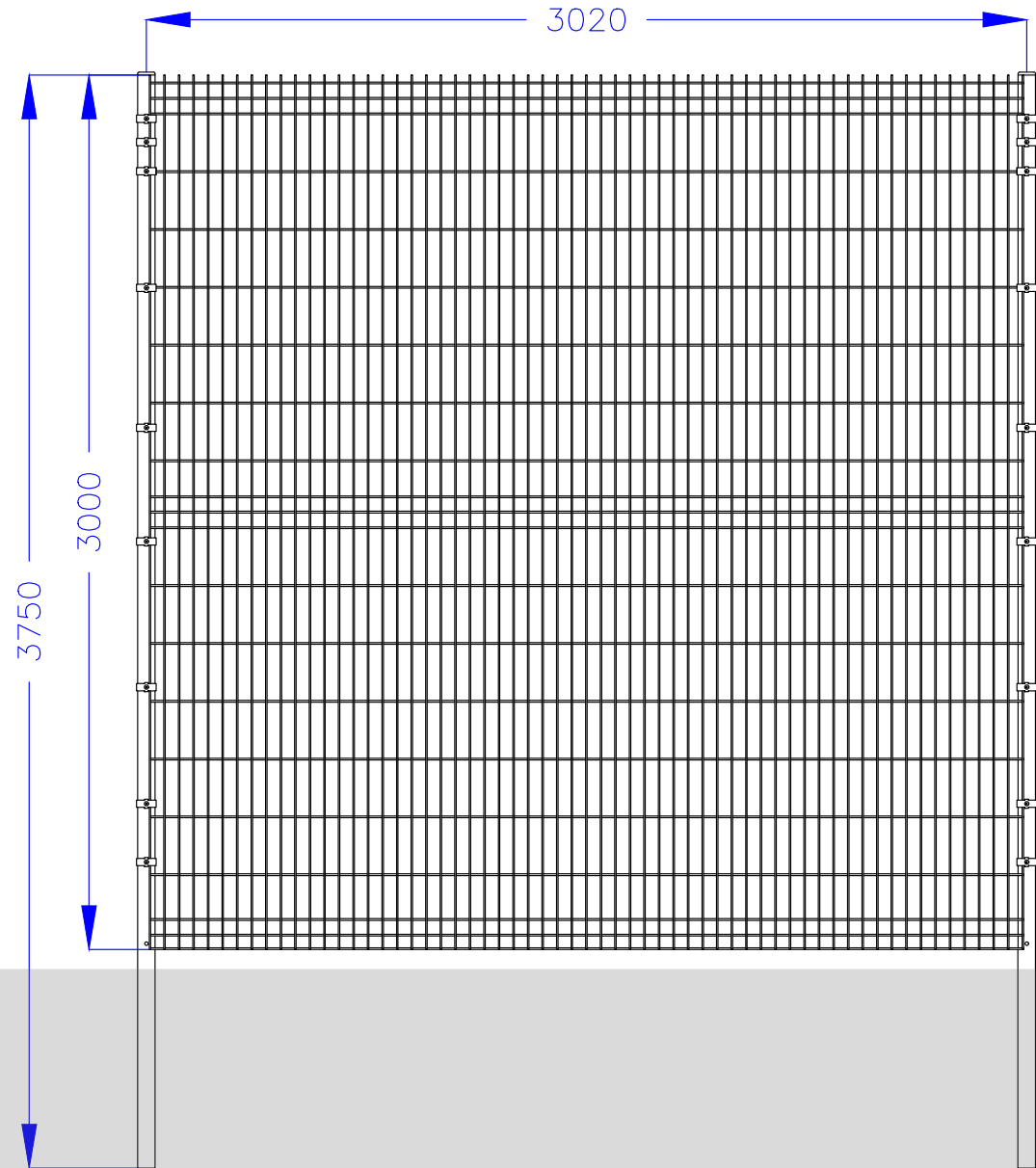
New fence TYPE A 3m green wire
