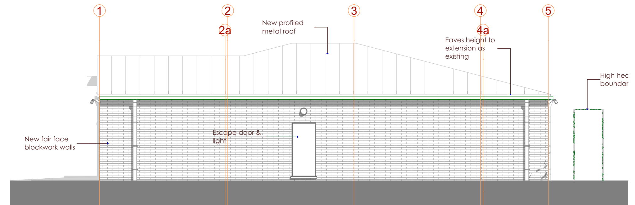
West Elevation
