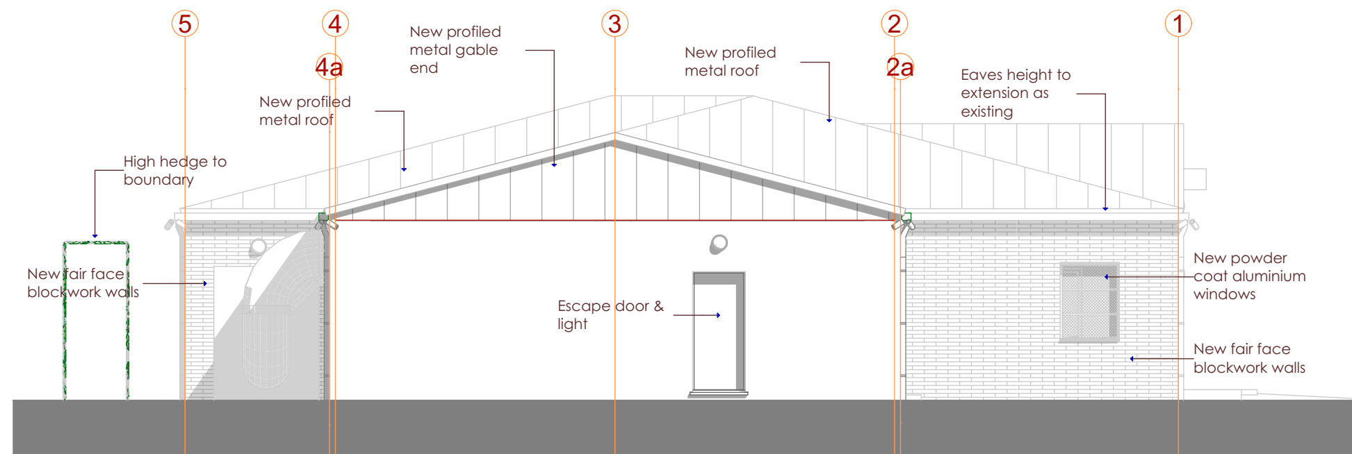
East Elevation
