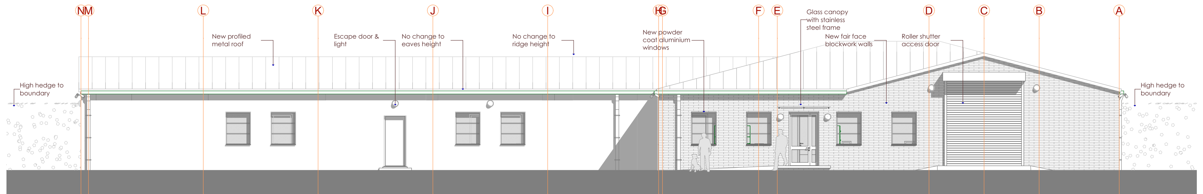
North Elevation
