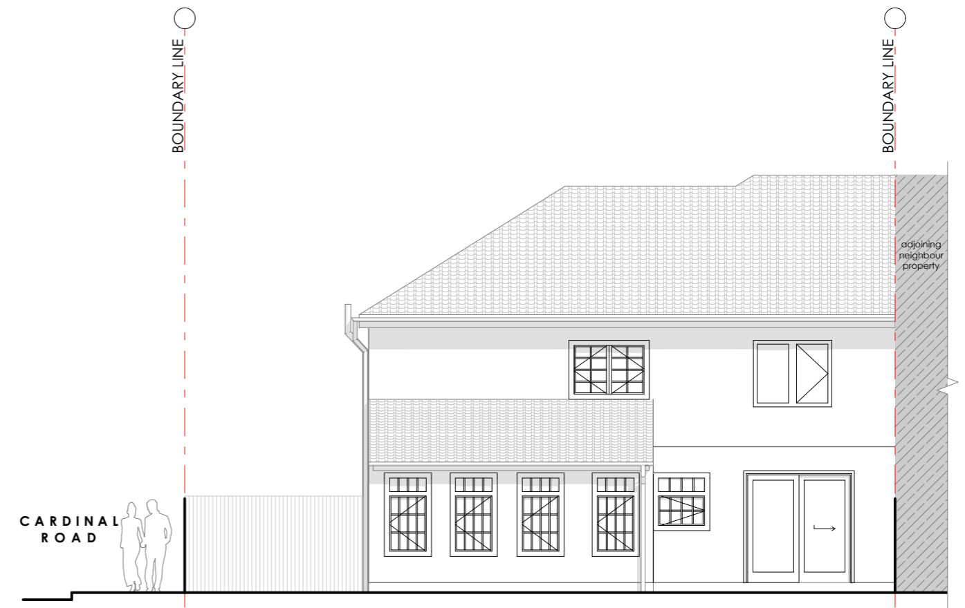
03 EXISTING NORTHERN ELEVATION (REAR) 1:100
