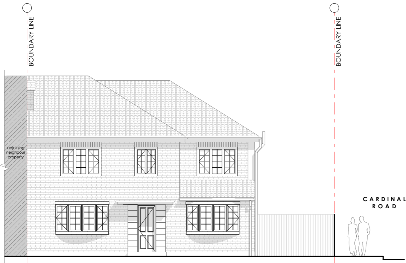
01 EXISTING SOUTHERN ELEVATION (FRONT) 1:100
