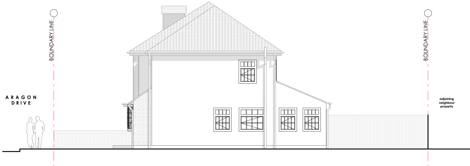
02 EXISTING EASTERN ELEVATION (SIDE) 1:100
