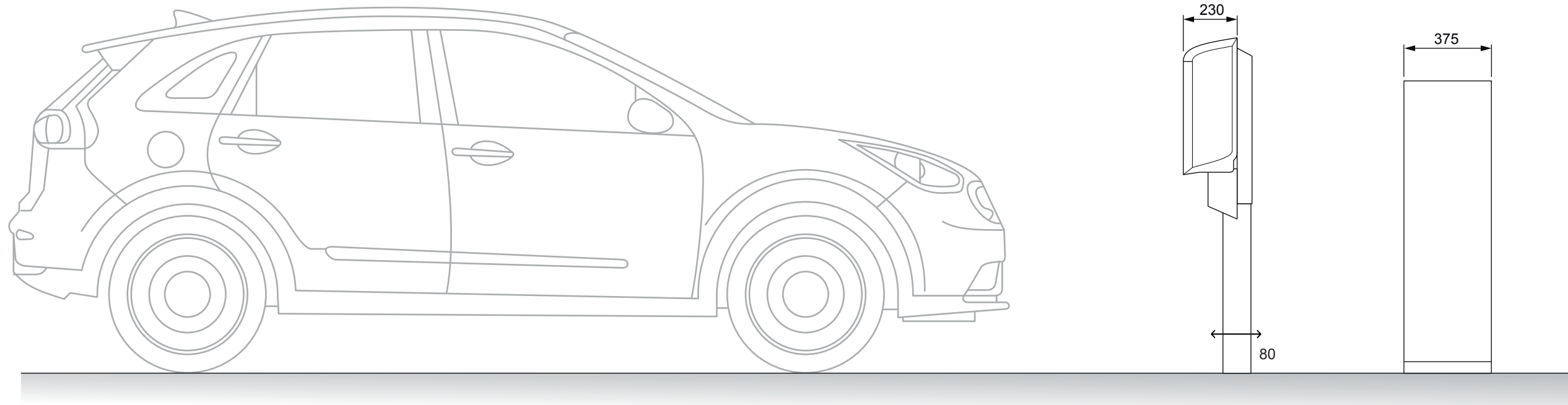
SIDE ELEVATION
