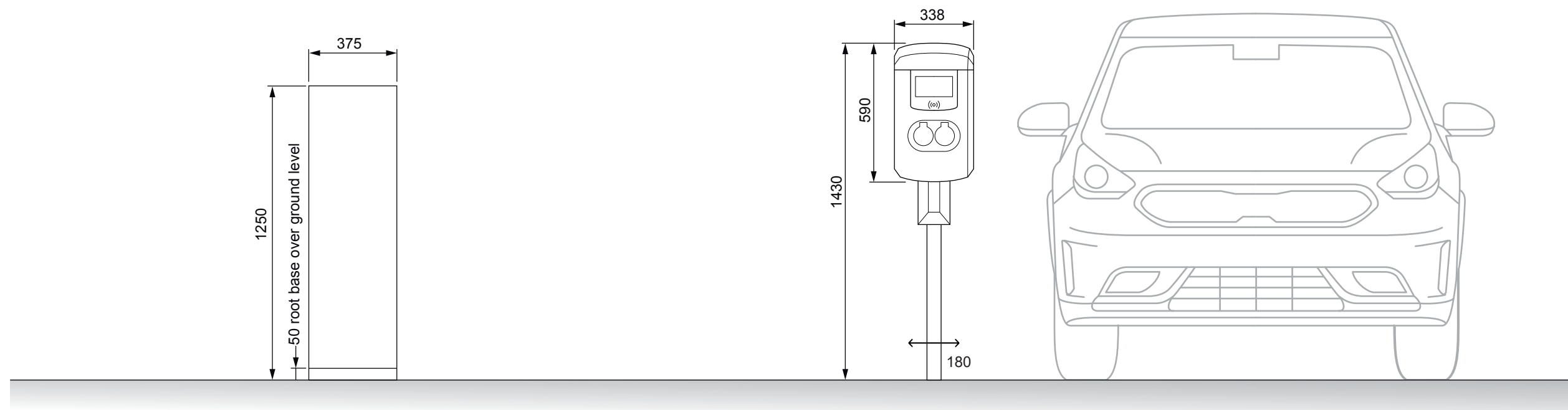
FRONT ELEVATION
