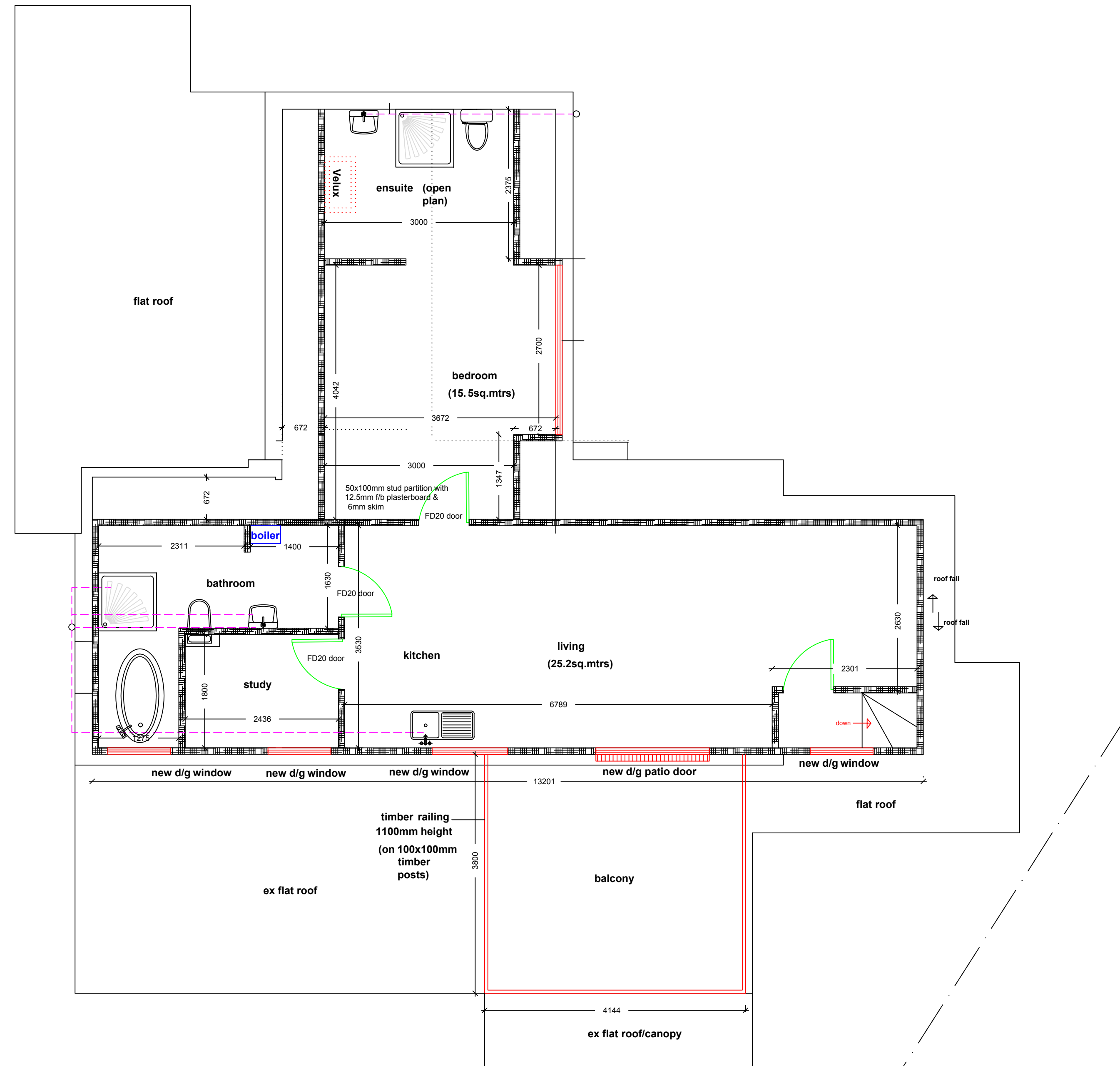
existing loft plan 1:50
