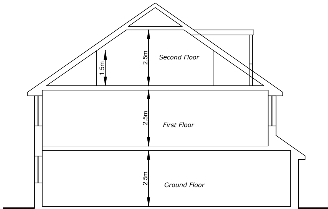
Typical Section
