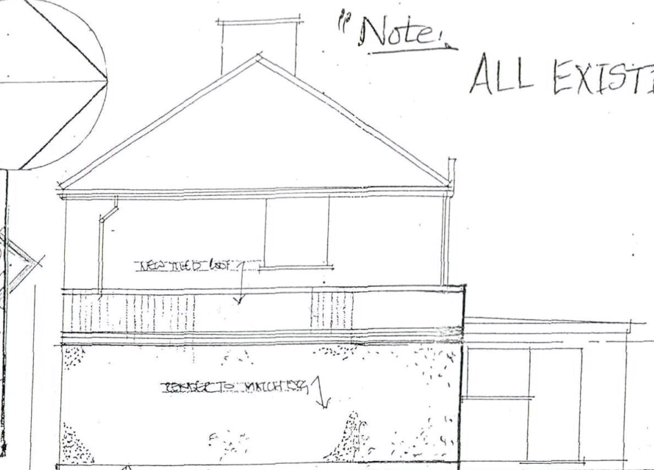
(L-R). EXISTING SIDE ELEVATION (1:100)
