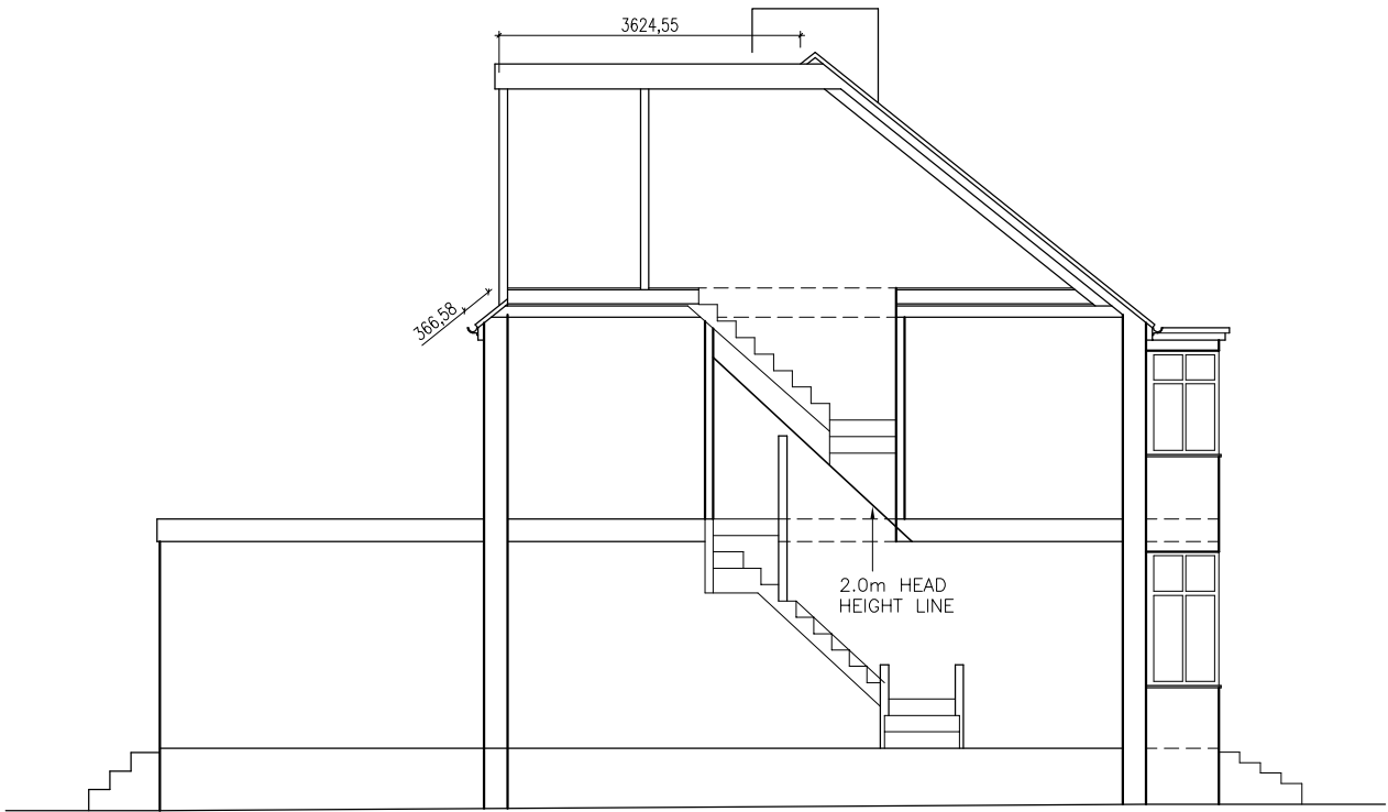
PROPOSED CROSS-SECTION OF STAIR
