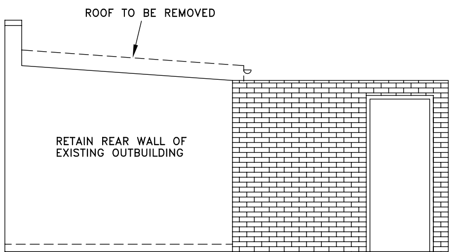
PROPOSED REAR WALL ELEVATION FACING THE HOUSE
