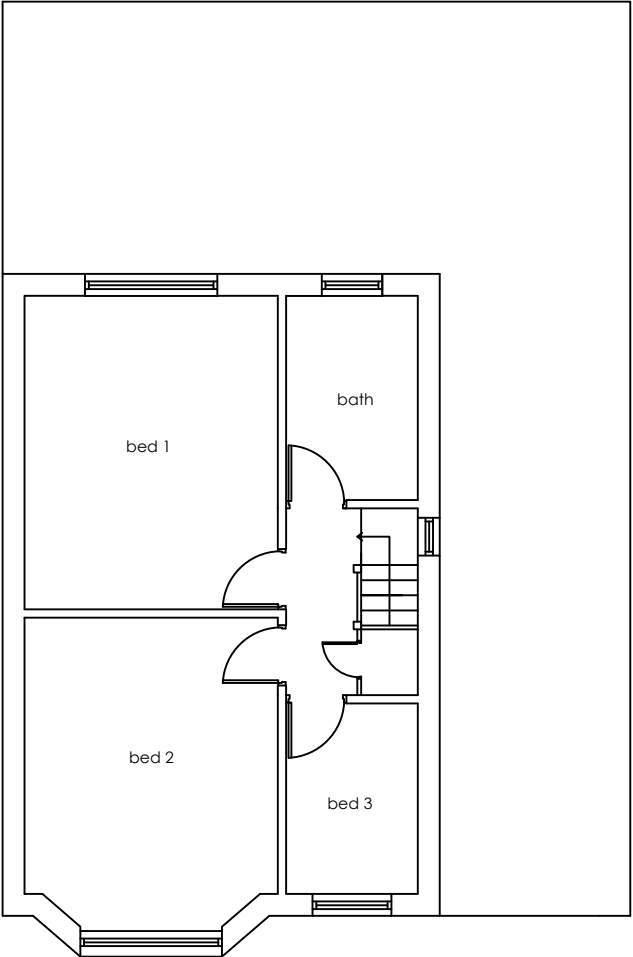
First Floor as Existing 1:100
