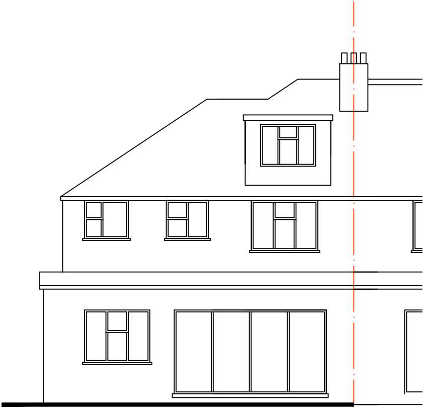
Rear Elevation as Proposed 1:100
