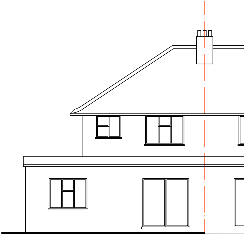
Rear Elevation as Existing 1:100
