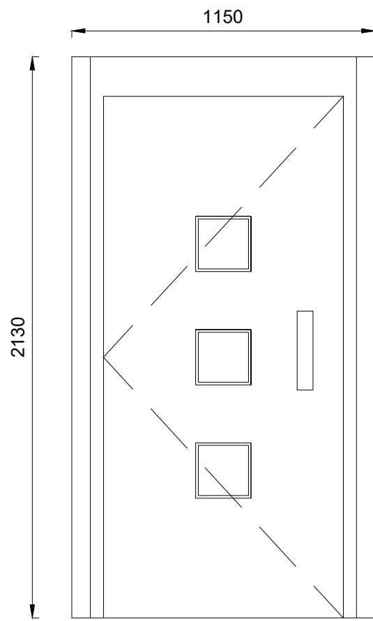
COMMON ENTRANCE DOOR no. 5 uPVC DOOR
