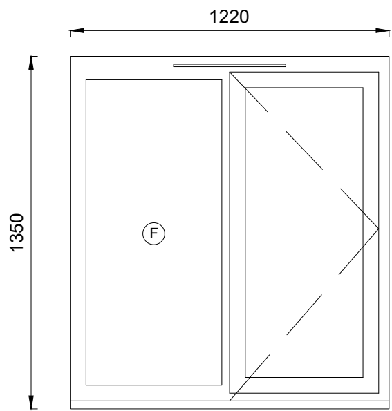
WINDOW nos. 1 + 40 uPVC WINDOW SIDE HUNG CASEMENT
