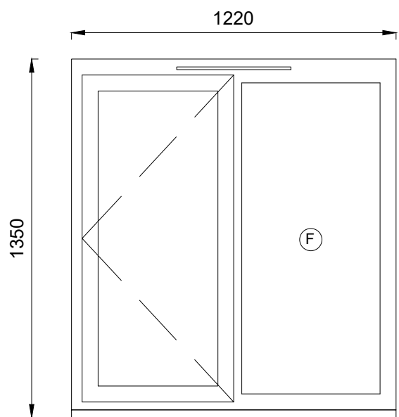
WINDOW nos. 9 + 47 uPVC WINDOW SIDE HUNG CASEMENT
