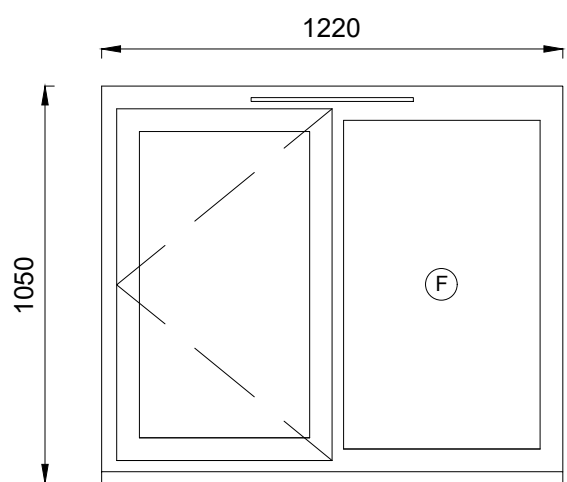
WINDOW nos. 25,27,29,57 + 65 uPVC WINDOW SIDE HUNG CASEMENT
