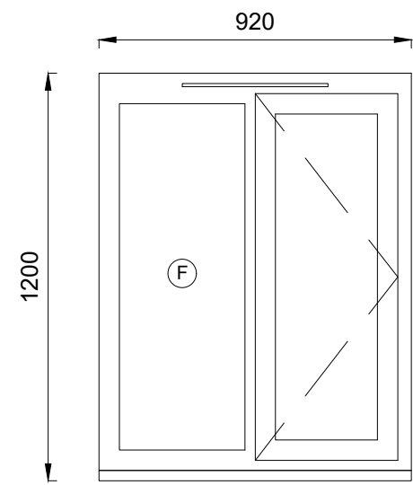
WINDOW nos. 6 + 14 uPVC WINDOW SIDE HUNG CASEMENT
