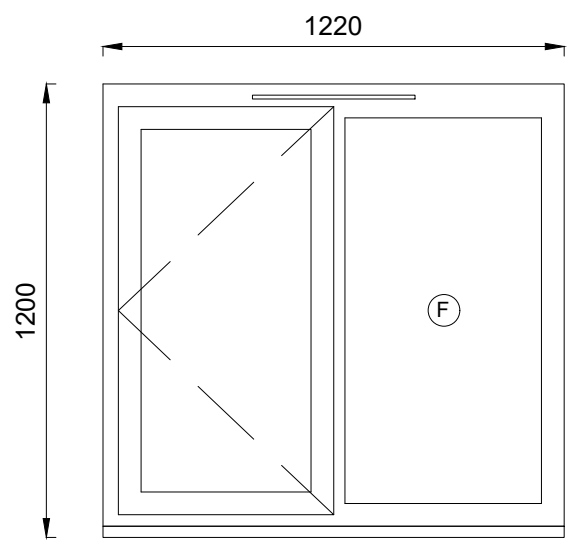
WINDOW nos. 17,48,51,52,56 + 61 uPVC WINDOW SIDE HUNG CASEMENT
