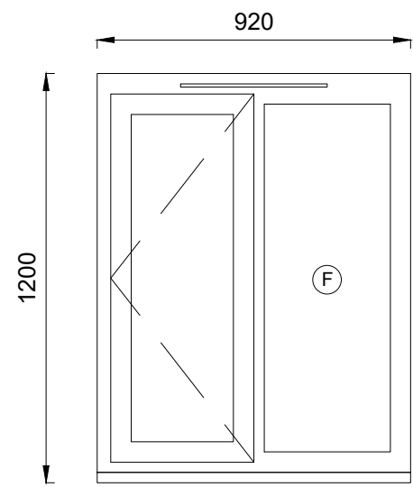
WINDOW nos. 4 + 13 uPVC WINDOW SIDE HUNG CASEMENT
