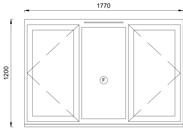
WINDOW nos. 3,7,12,15,42,45,50 + 54 uPVC WINDOW SIDE HUNG CASEMENT
