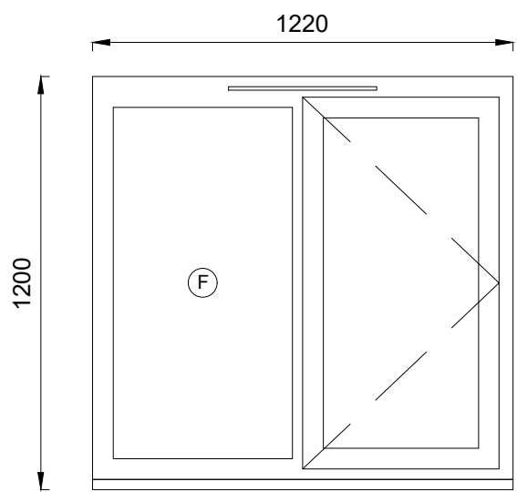
WINDOW nos. 10,43,44 + 53 uPVC WINDOW SIDE HUNG CASEMENT
