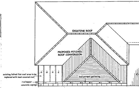
ROOF LAYOUT
