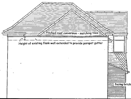
FLANK ELEVATION FACING NO. 38
