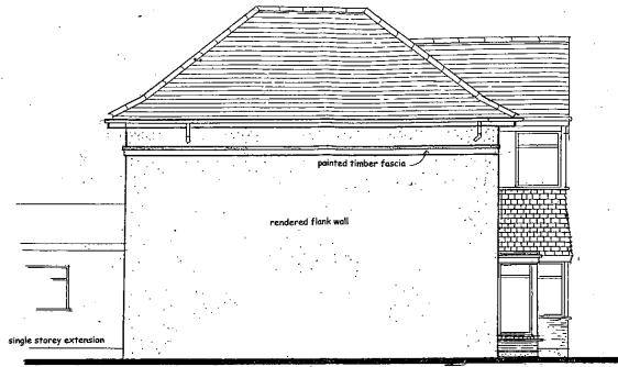
FLANK ELEVATION FACING NO. 38
