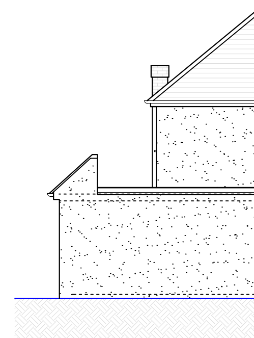
○ Side Elevation 1 Partial 1:100
