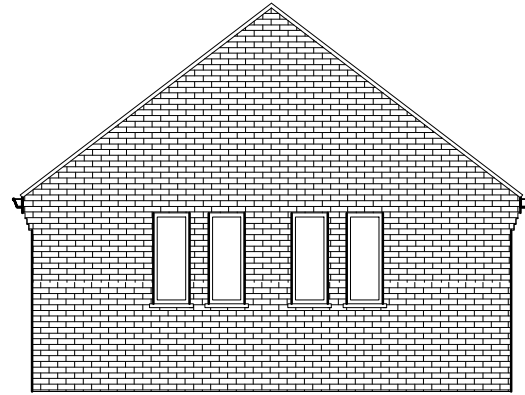
EXISTING LEFT SIDE ELEVATION
