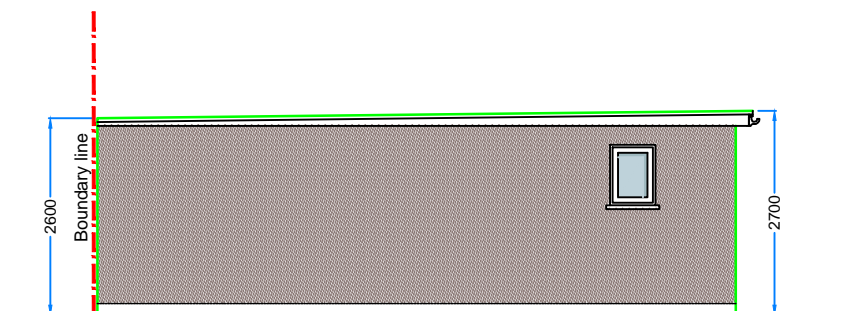
EXISTING AND PROPOSED OUTBUILDING FLANK ELEVATION
