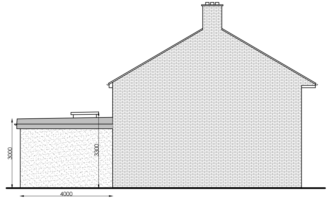
PROPOSED OPPOSITE SIDE ELEVATION
