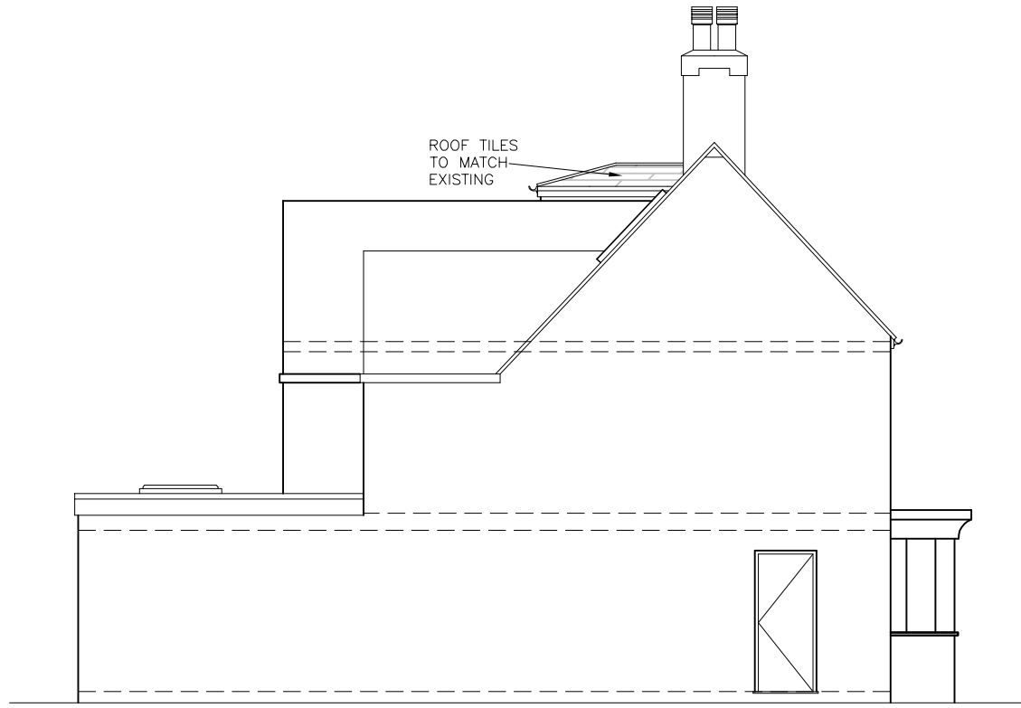
PROPOSED OTHER SIDE ELEVATION
