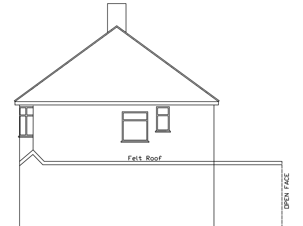
Existing Side Elevation(From No.6 Chatsworth Rd)
