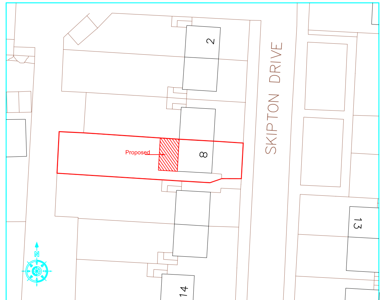
Block Plan 1:500
