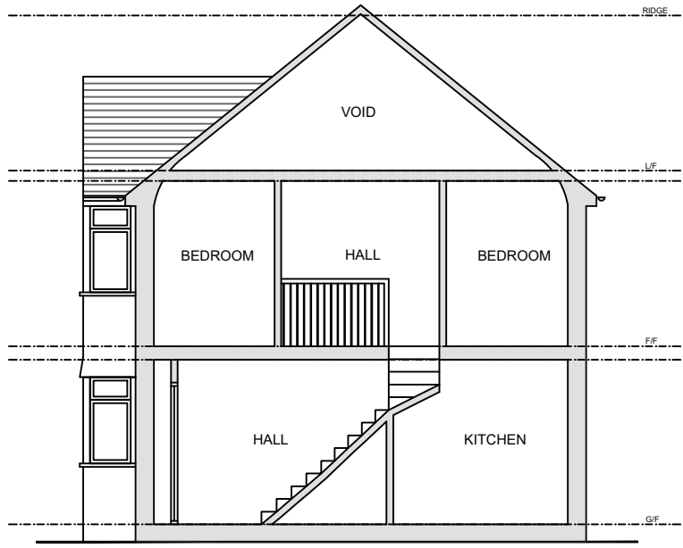
EXISTING SIDE SECTION
