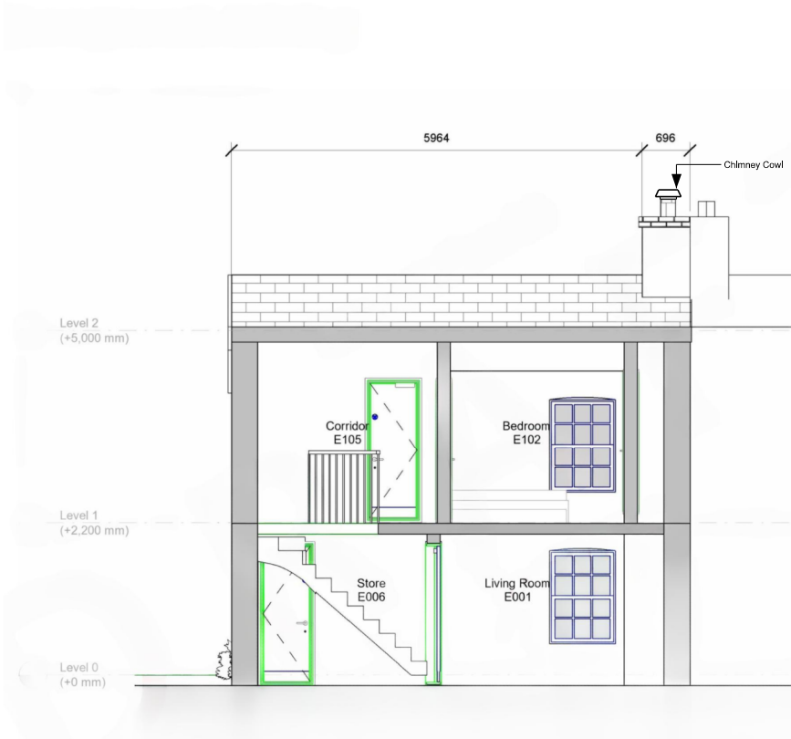
Proposed Section 02
