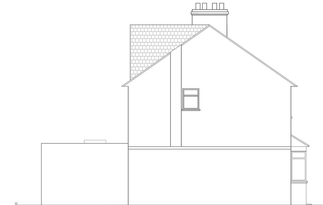
SIDE (SW) ELEVATION
