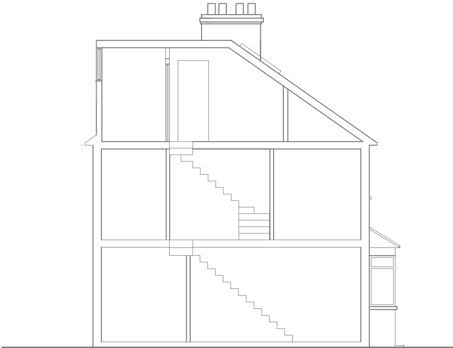
PROPOSED SECTION
