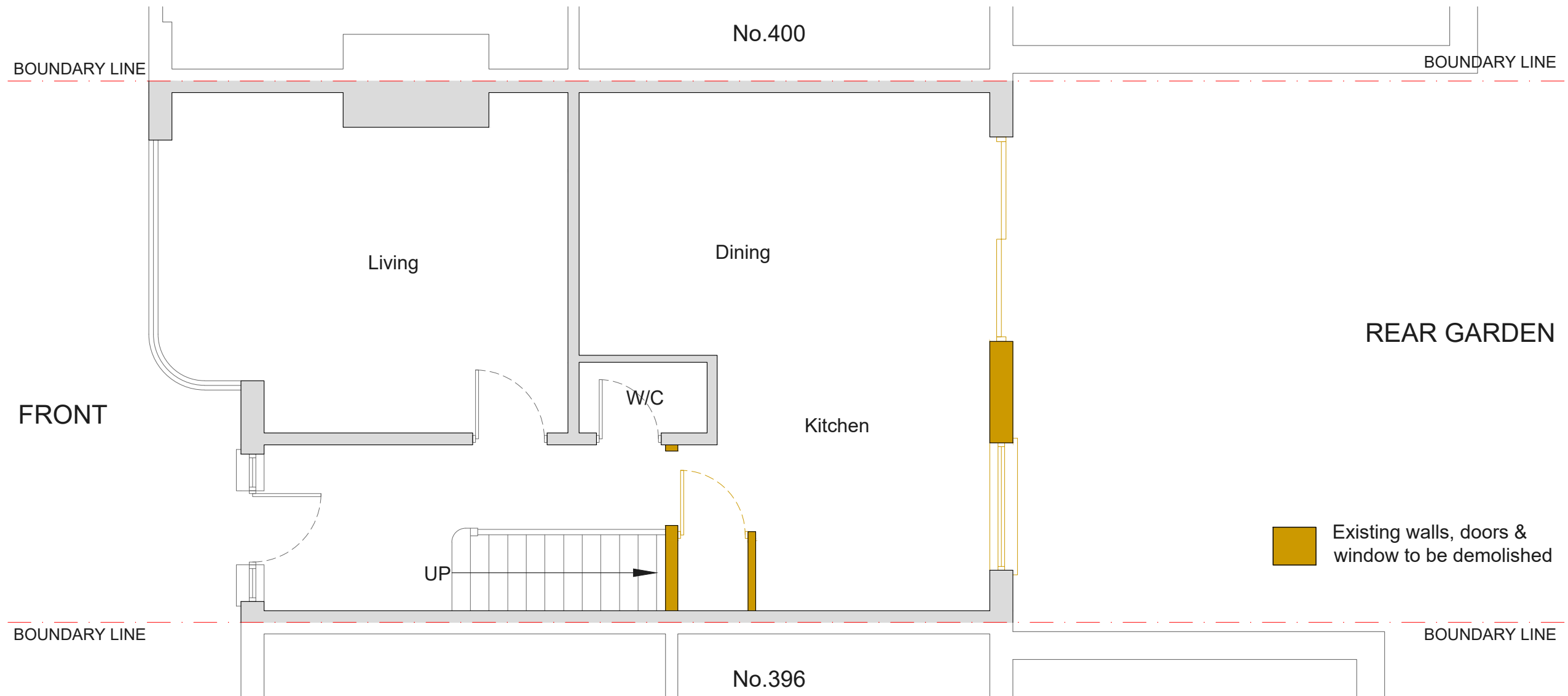
EXISTING GROUND FLOOR PLAN SCALE 1:50
