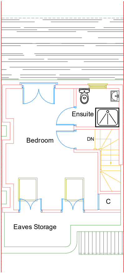
Proposed Loft Floor Plan
