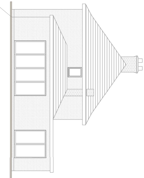
As Proposed Side Elevation facing crossroad
