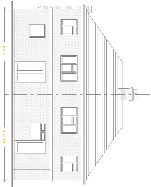
As Existing Rear Elevation
