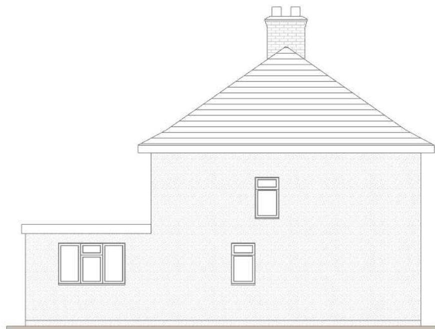
As Existing Side Elevation facing no.67
