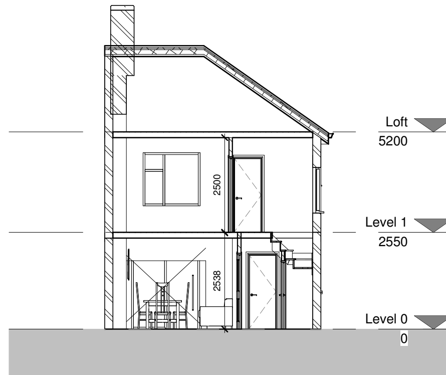
3 Proposed - Section 1 1 : 100
