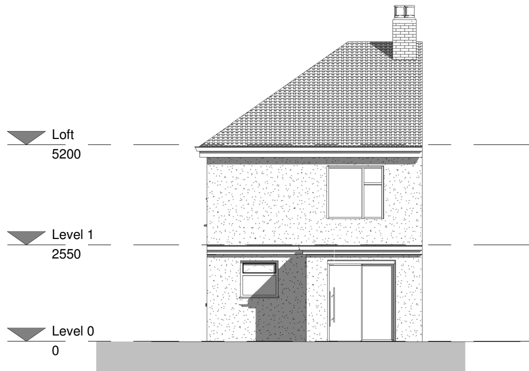
1 Rear elevation - Existing 1 : 100
