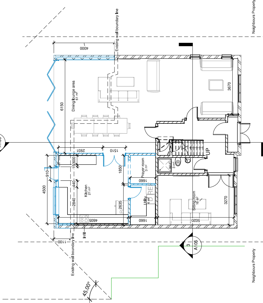
00 - Proposed 2 : 1 : 100
