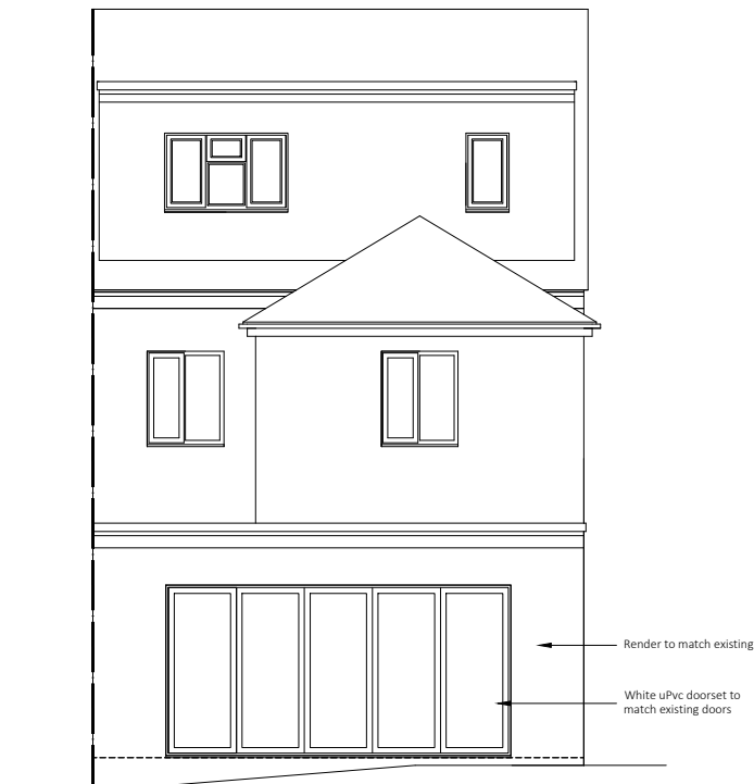
REAR ELEVATION
