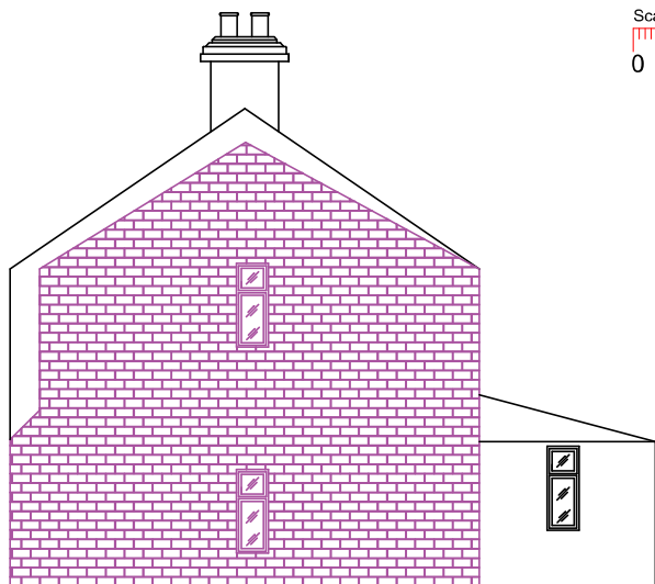
PROPOSED RIGHT SIDE ELEVATION
